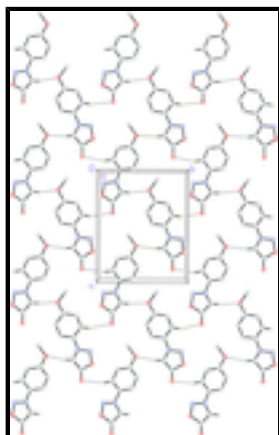
Fig. 2. The crystal structure of the title compound, viewed along the a axis, showing a two-dimensional sheet parallel to the bc plane. H atoms not involved in intermolecular hydrogen bonds (dashed lines) have been omitted for clarity.
